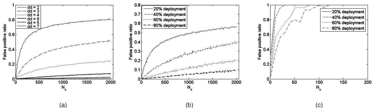
Fig. 9. The false positive ratios of AD with gradual deployment: (a) for various deployment depths, (b) dd = 2 and uniformly random deployment for all other subnets in the Internet, and (c) the victim's edge router supports AD, subnets at deployment depths one and two from the victim do not support AD, and uniformly random deployment for all other subnets in the Internet.
